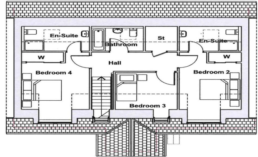
First Floor 1:100
